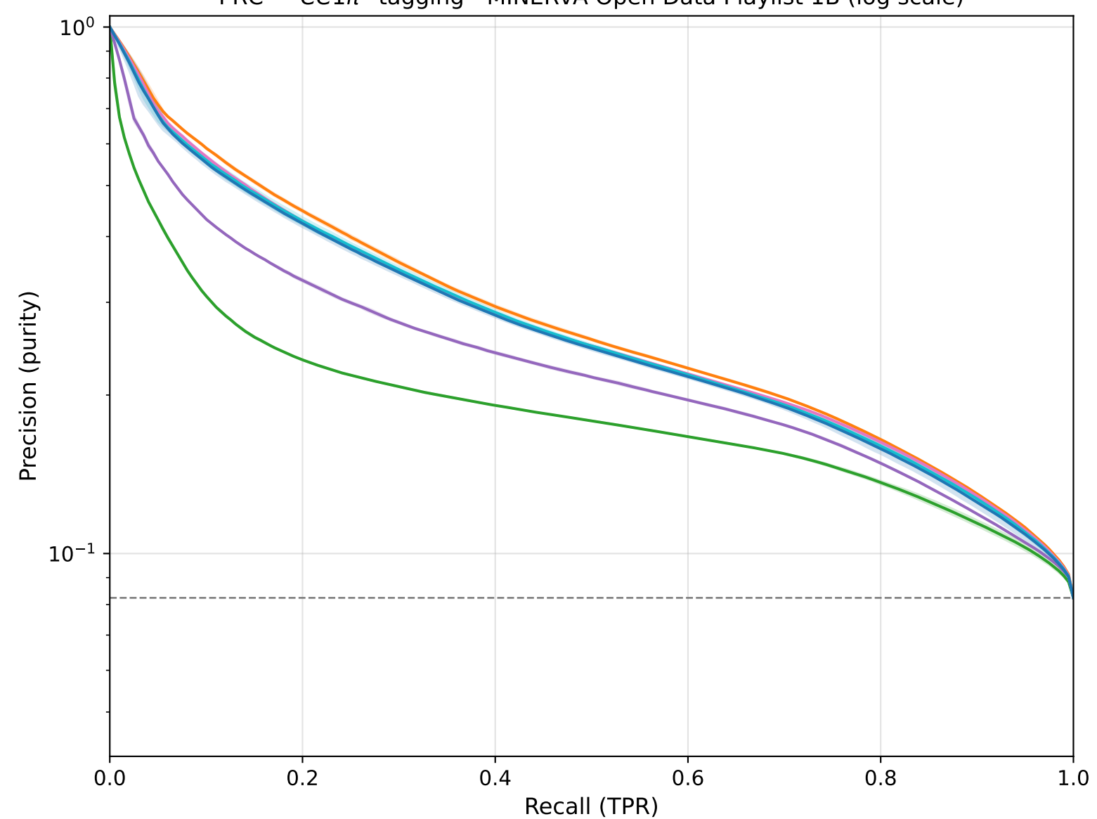
PRC — CC1\pi^0 tagging - MINERvA Open Data Playlist 1B (log scale)
