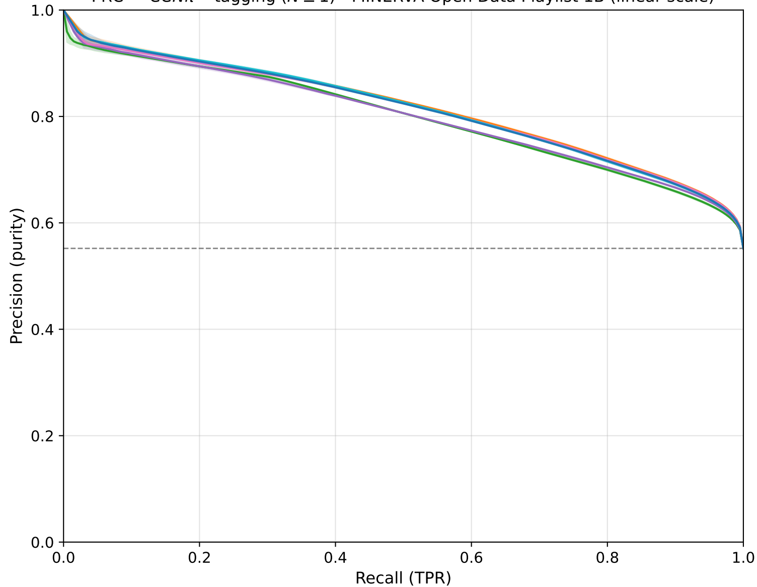
PRC — CCN\pi^\pm tagging ( N \geq 1 ) - MINERvA Open Data Playlist 1B (linear scale)
