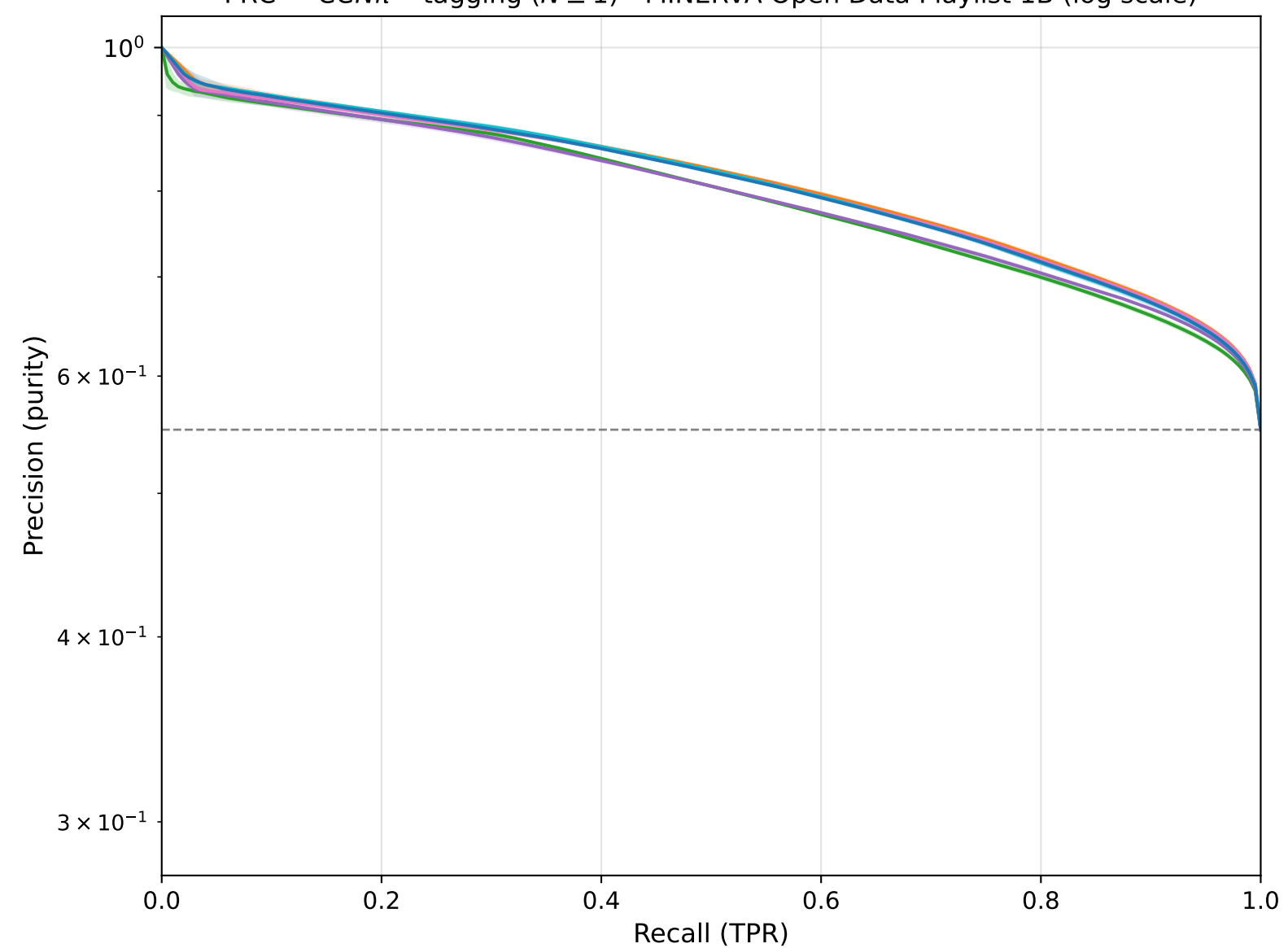
PRC — CCN\pi^\pm tagging ( N \geq 1 ) - MINERvA Open Data Playlist 1B (log scale)
