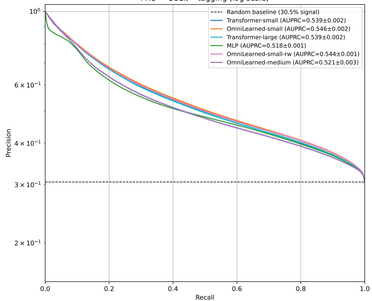
PRC — CC1\pi^\pm tagging (log scale)
