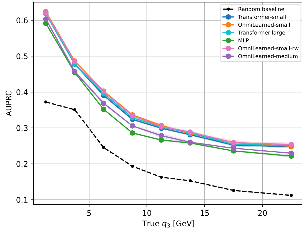
AUPRC vs. q_3
