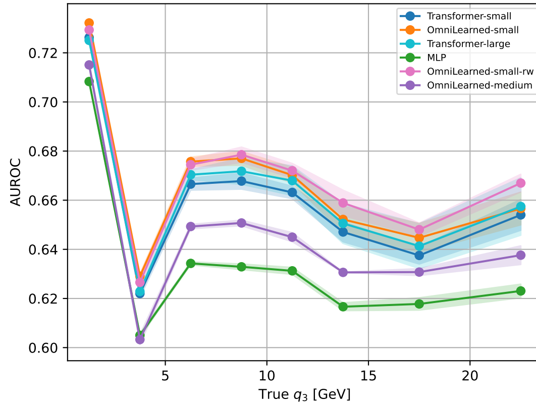
AUROC vs. q_3
