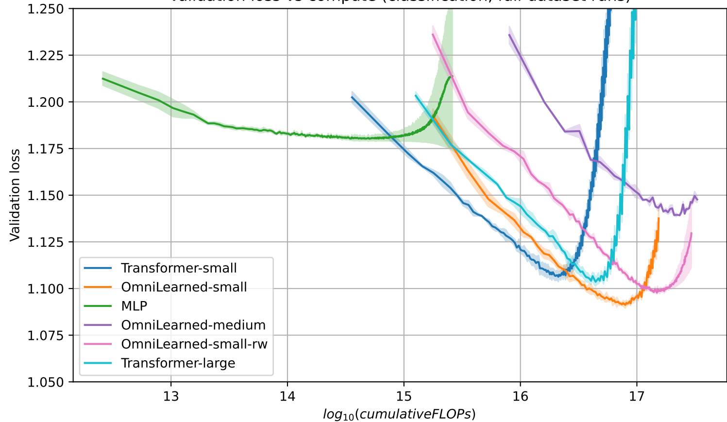
Validation loss vs compute (classification, full-dataset runs)
