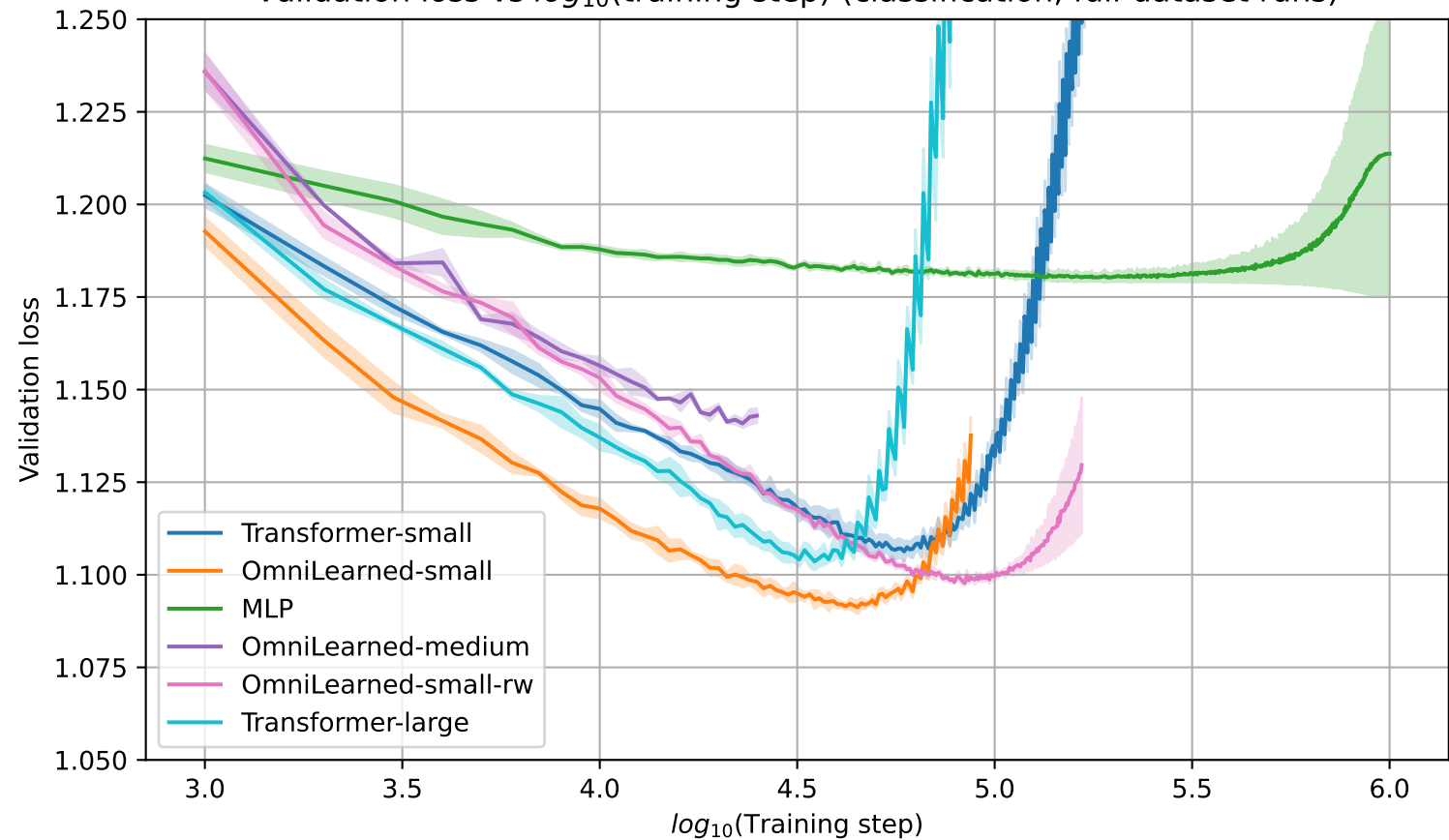
Validation loss vs \log_{10}(\text{training step}) (classification, full-dataset runs)
