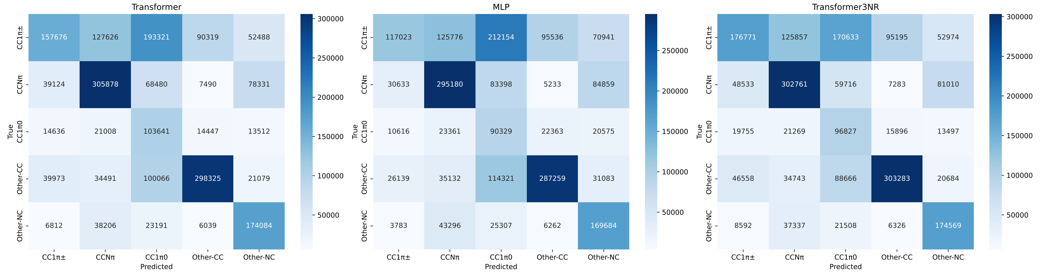
Confusion matrices (first run per model) — 1B
