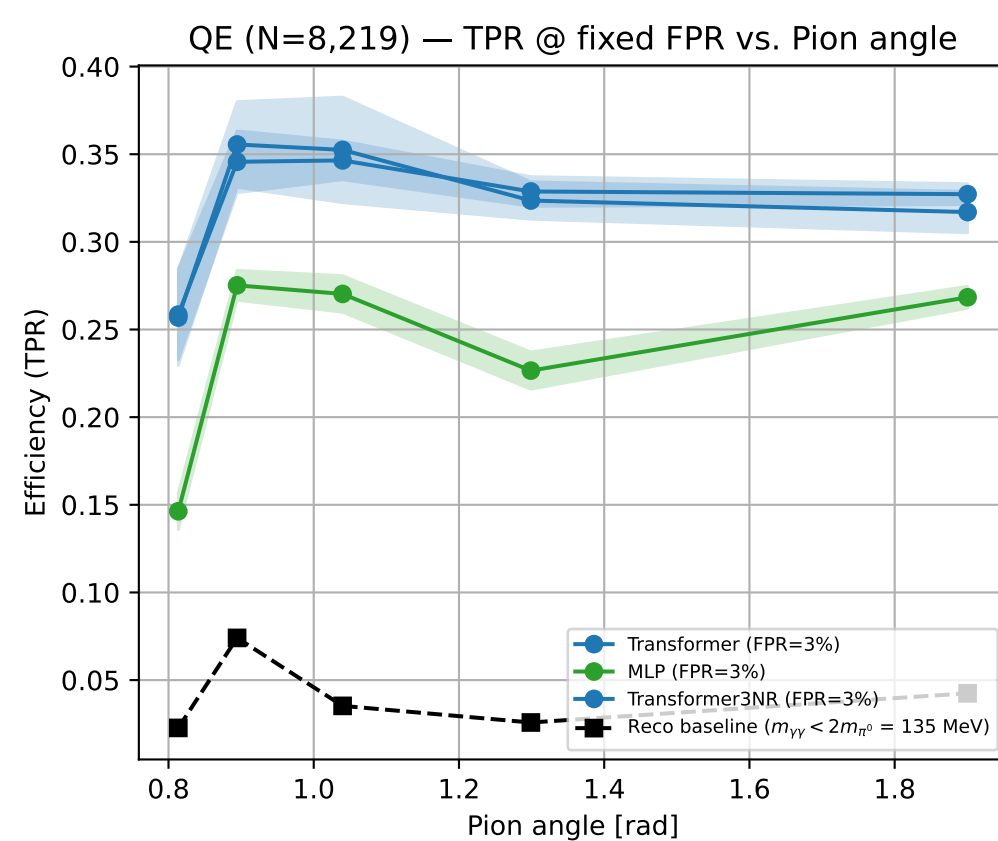
CC \pi^0 tagging vs. pion angle — by interaction type
