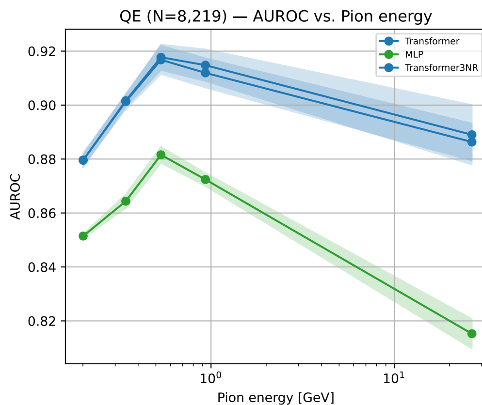
CC\pi^0 tagging vs. pion energy — by interaction type
