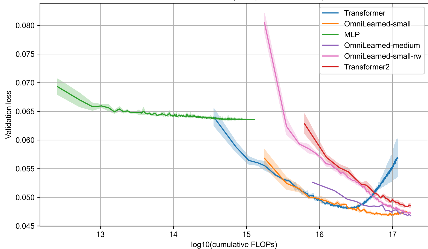
Validation loss vs compute (full-dataset runs)
