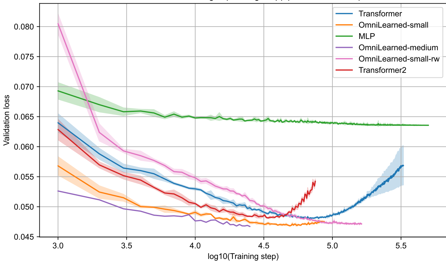
Validation loss vs log10(training step) (full-dataset runs)
