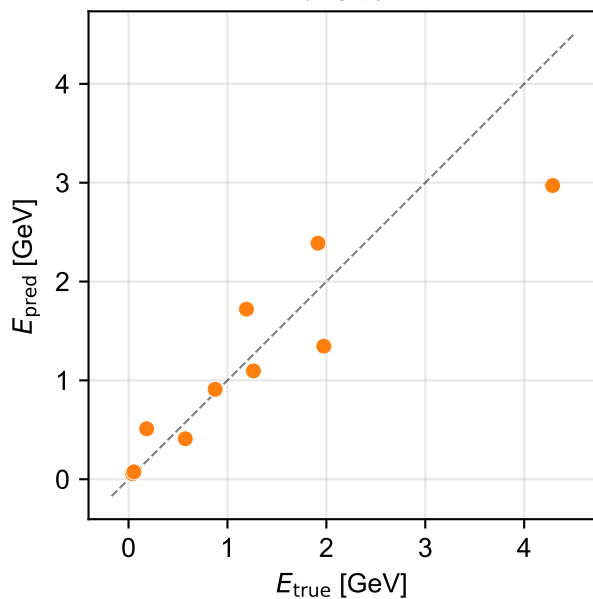
OmniLearned-small (Log1p)
