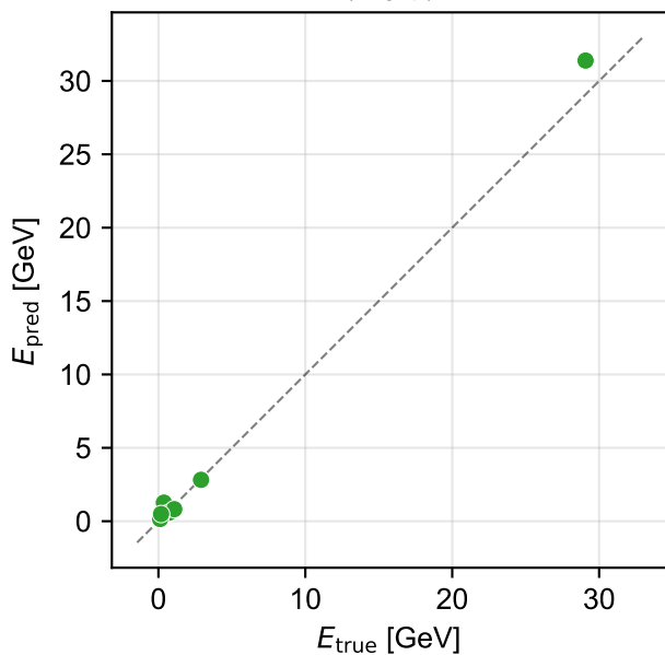
MLP (Log1p)
