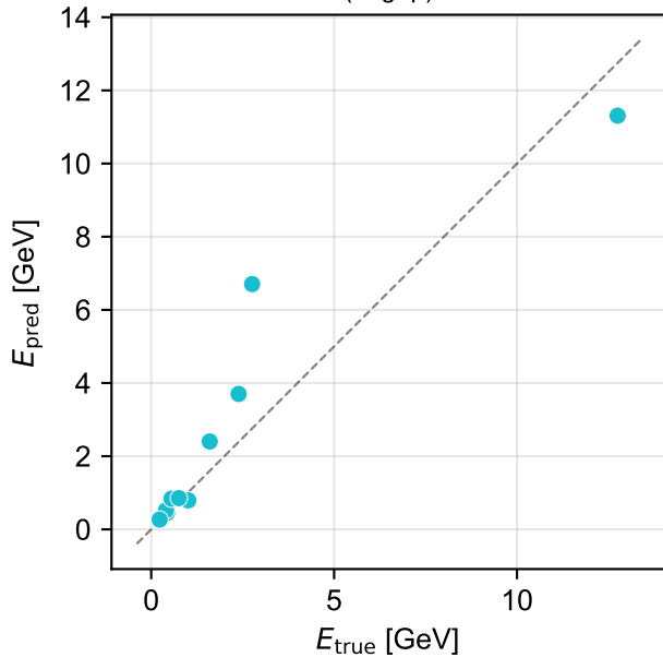
Transformer-large (Log1p)
