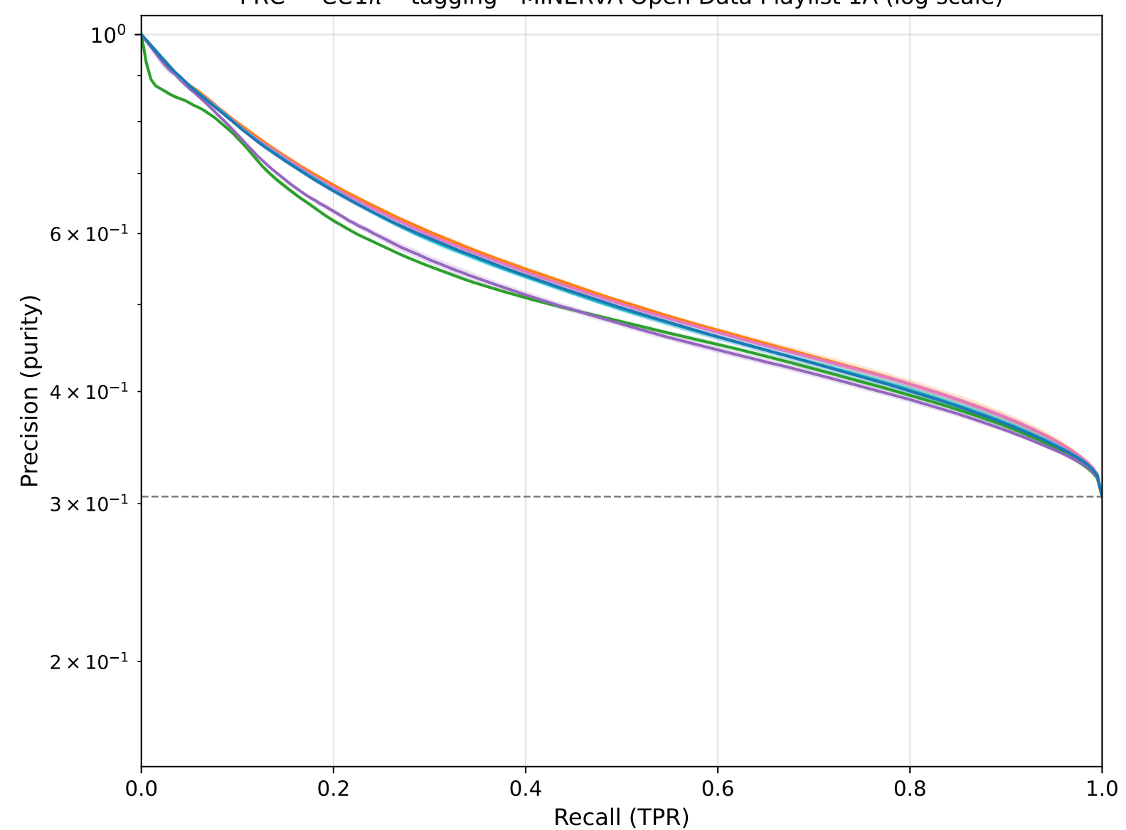
PRC — CC1\pi^\pm tagging - MINERvA Open Data Playlist 1A (log scale)
