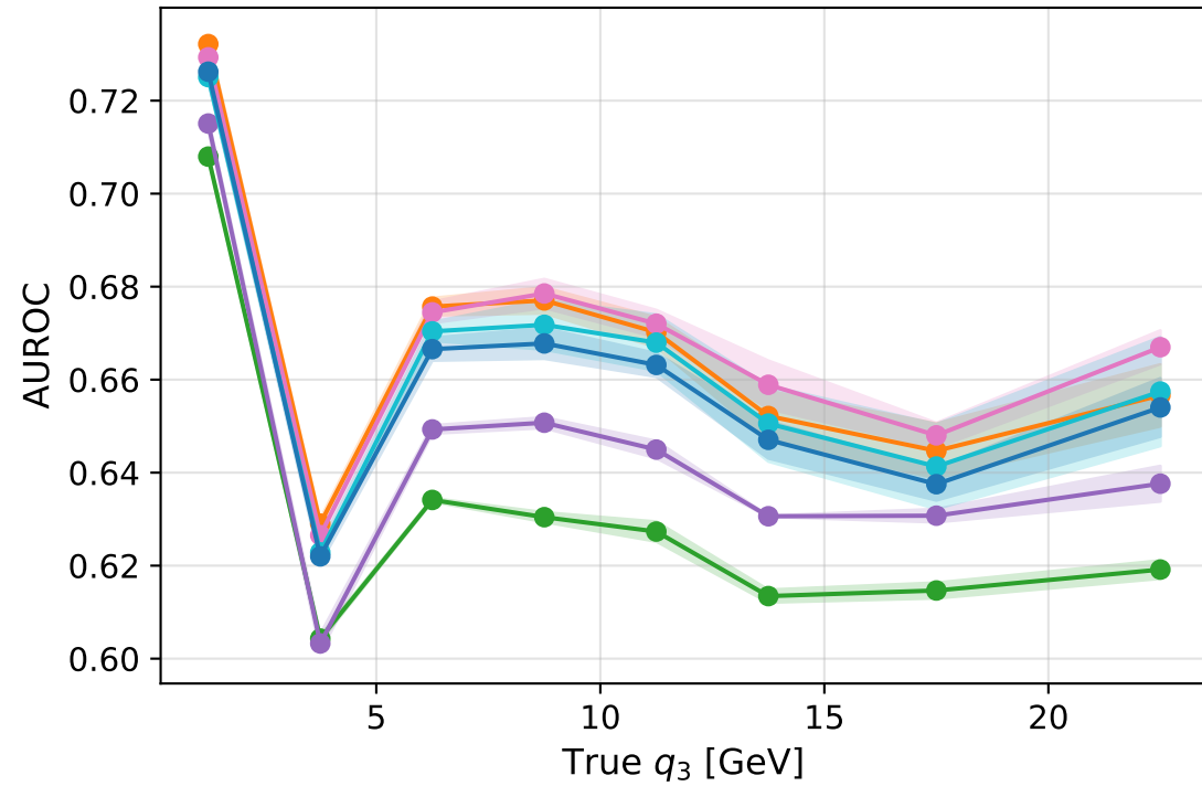
AUROC vs. True q_3
