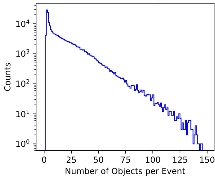
Number of reco objects
