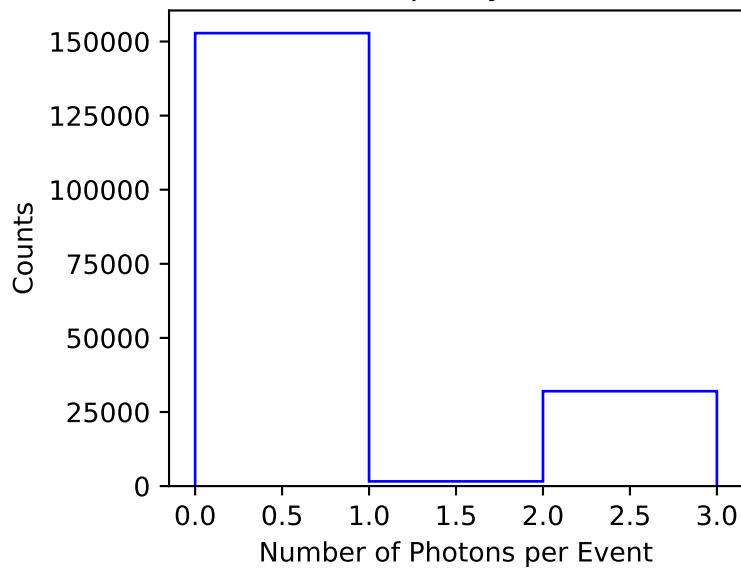
Photon Multiplicity Distribution
