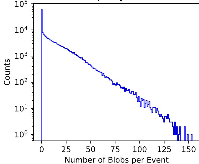
Blob Multiplicity Distribution
