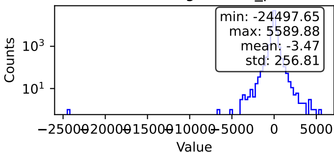
Photons - gamma1_px
