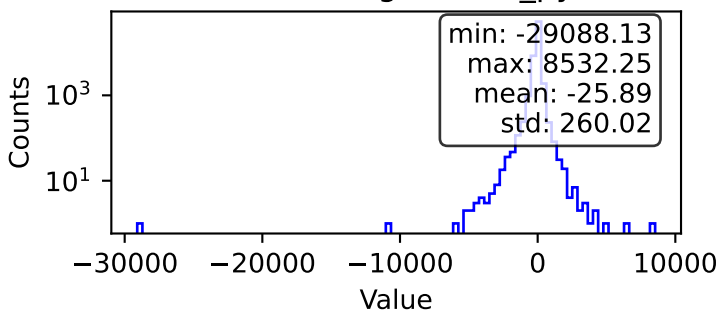
Photons - gamma1_py
