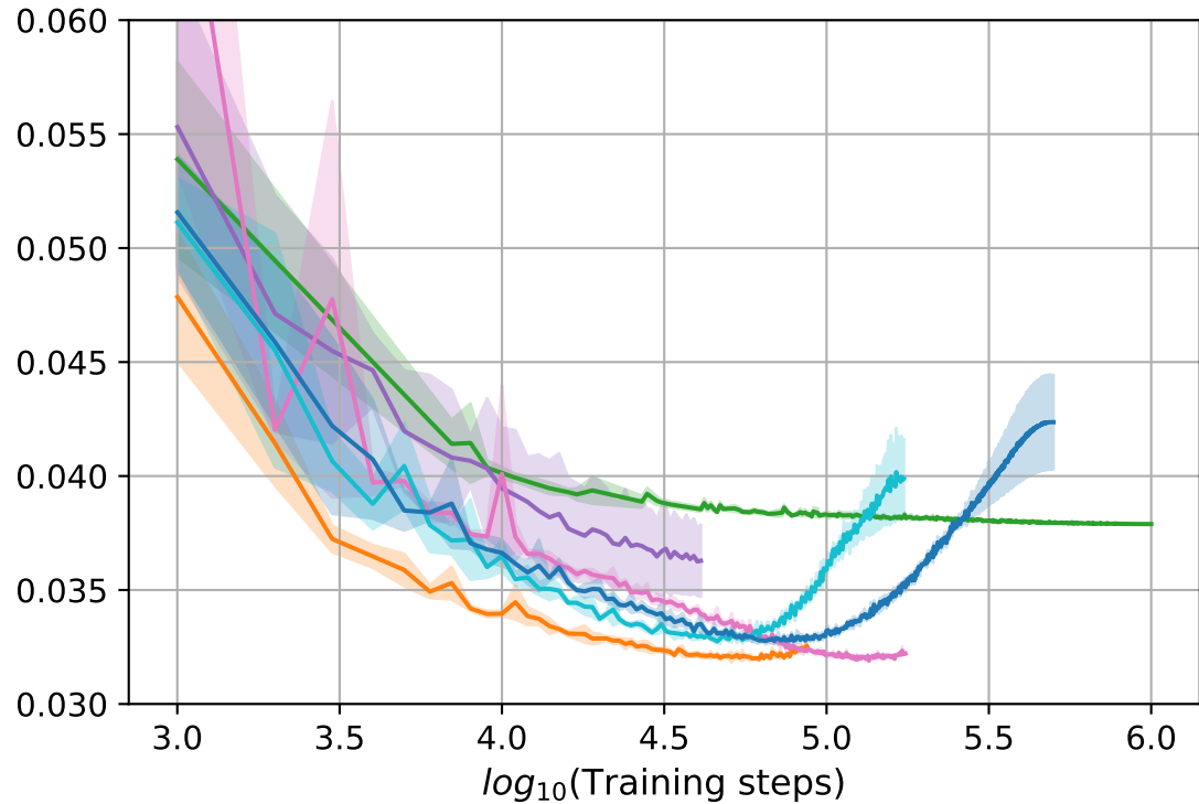
Regression
