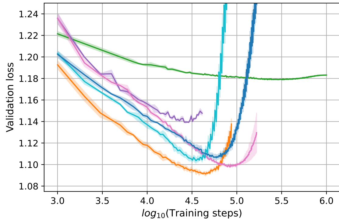
Classification
