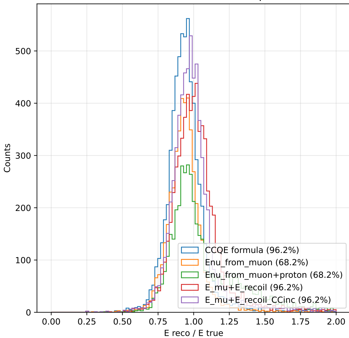
E reco / E true Distribution - 2p2h
