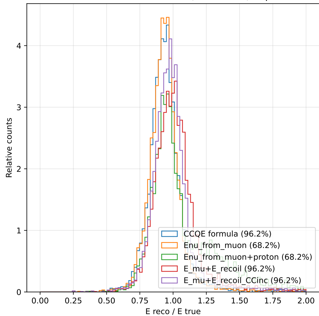
E reco / E true Distribution (normalized) - 2p2h
