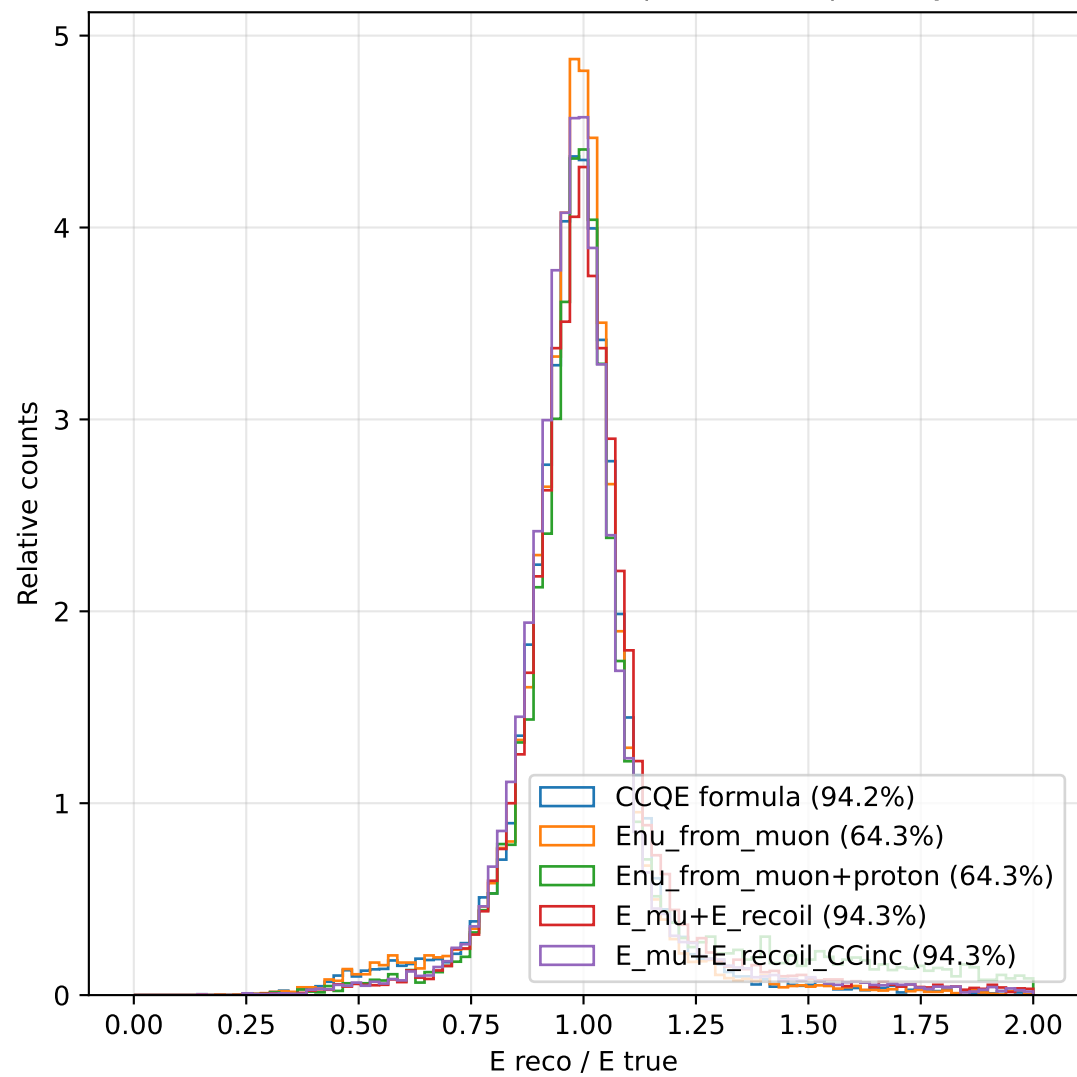
E reco / E true Distribution (normalized) - CCQE
