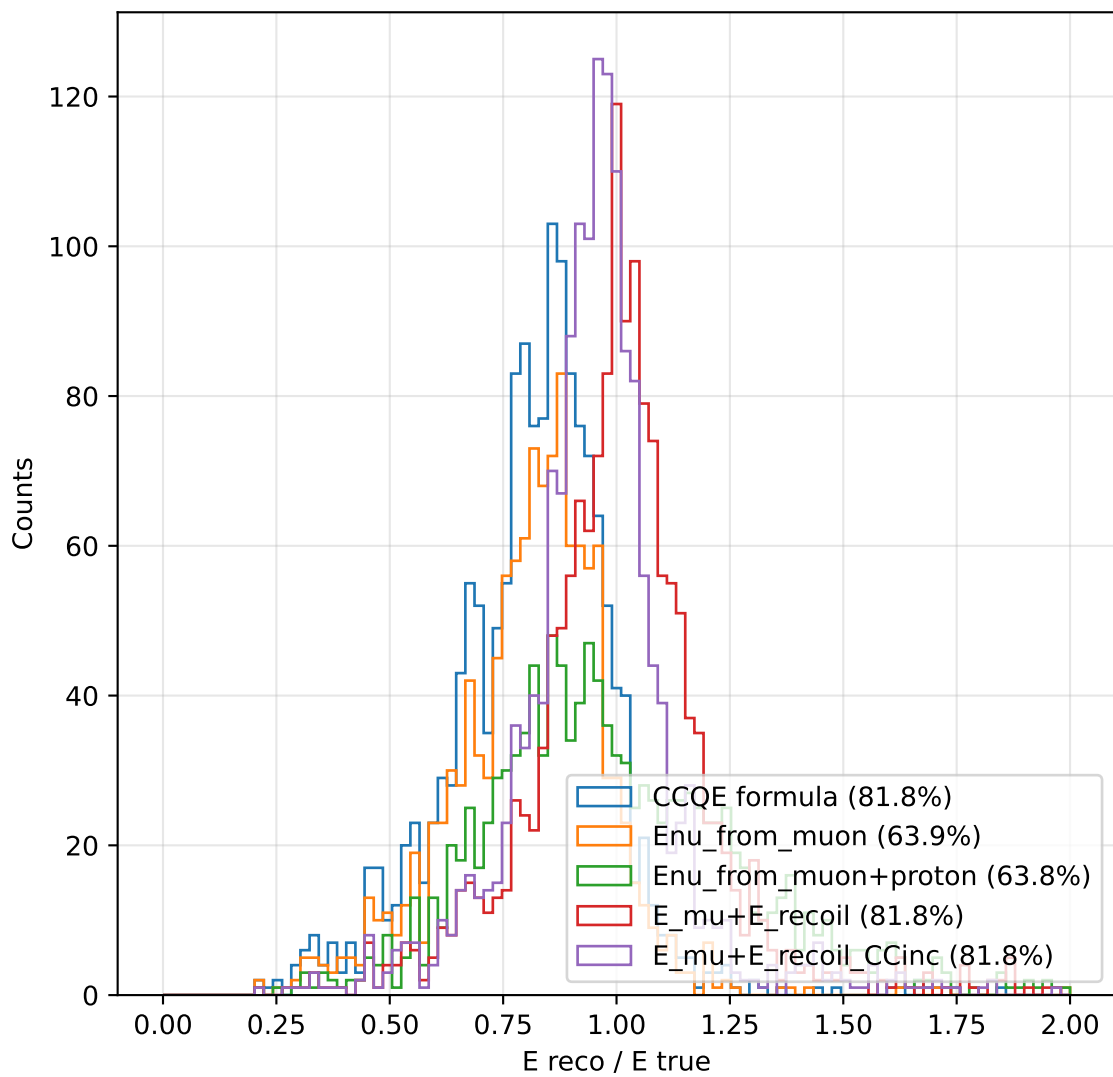
E reco / E true Distribution - Coherent
