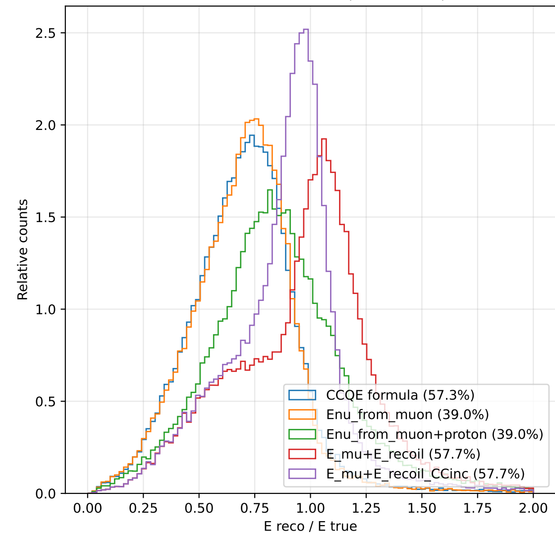
E reco / E true Distribution (normalized) - DIS
