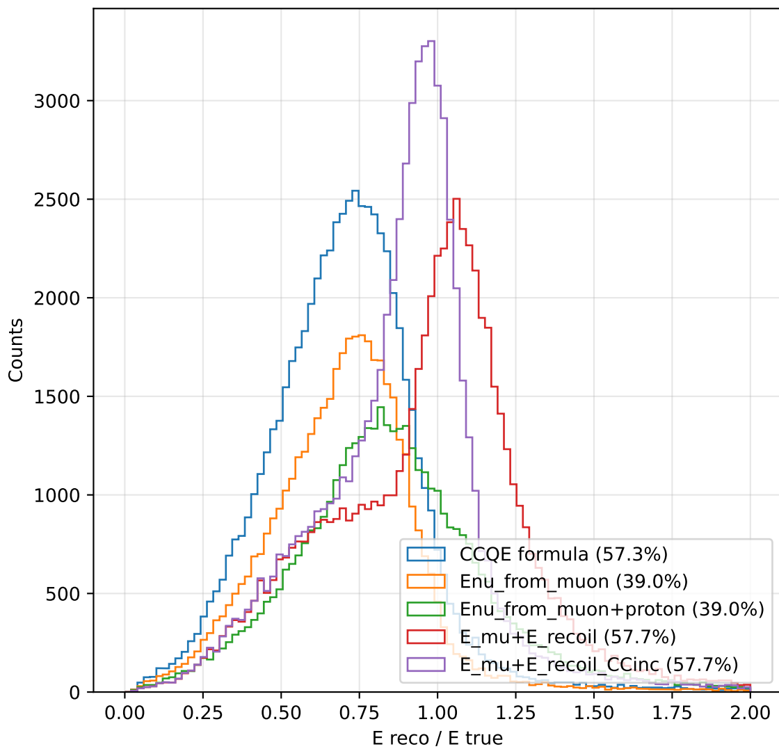
E reco / E true Distribution - DIS
