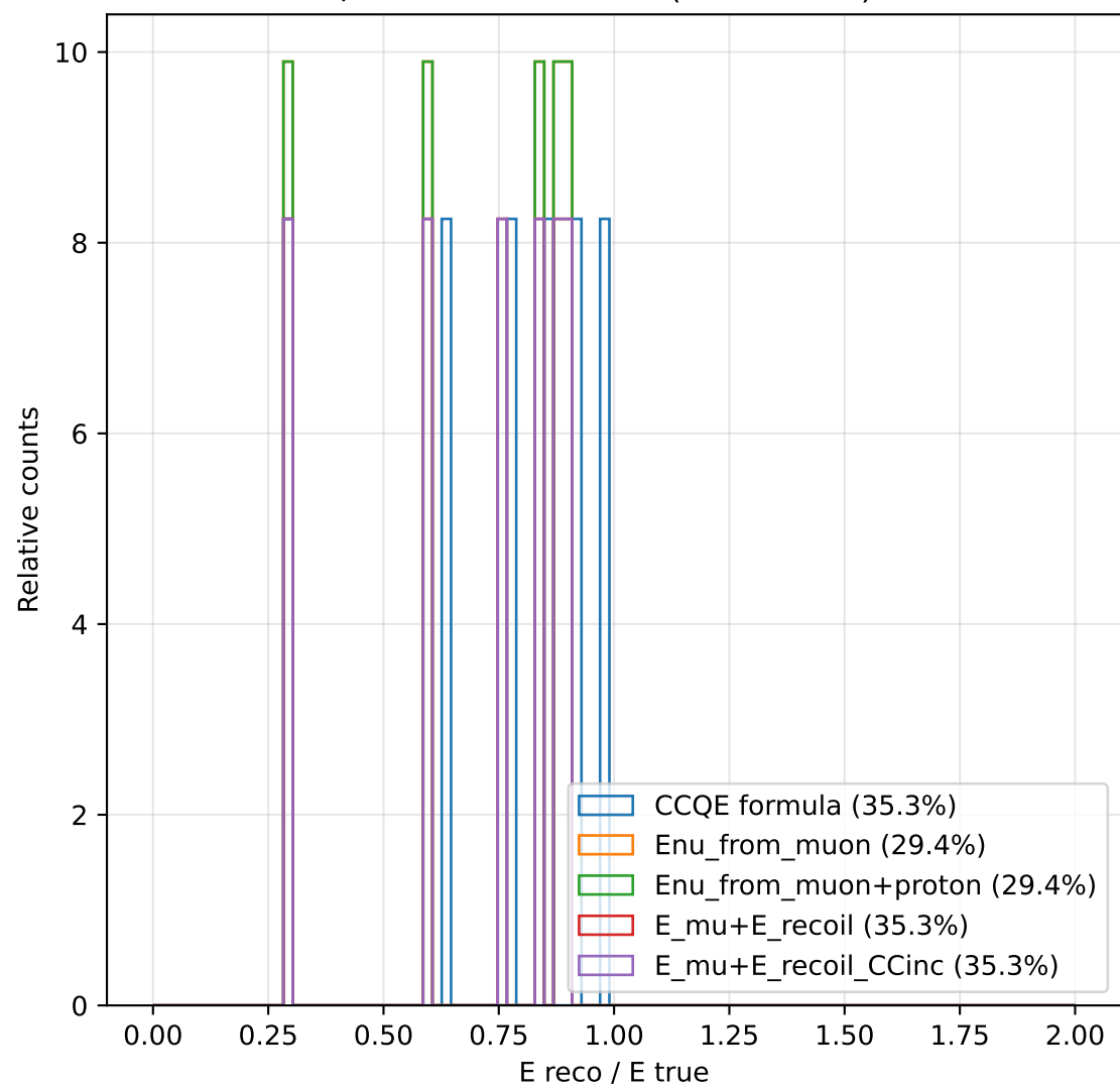
E reco / E true Distribution (normalized) - Other
