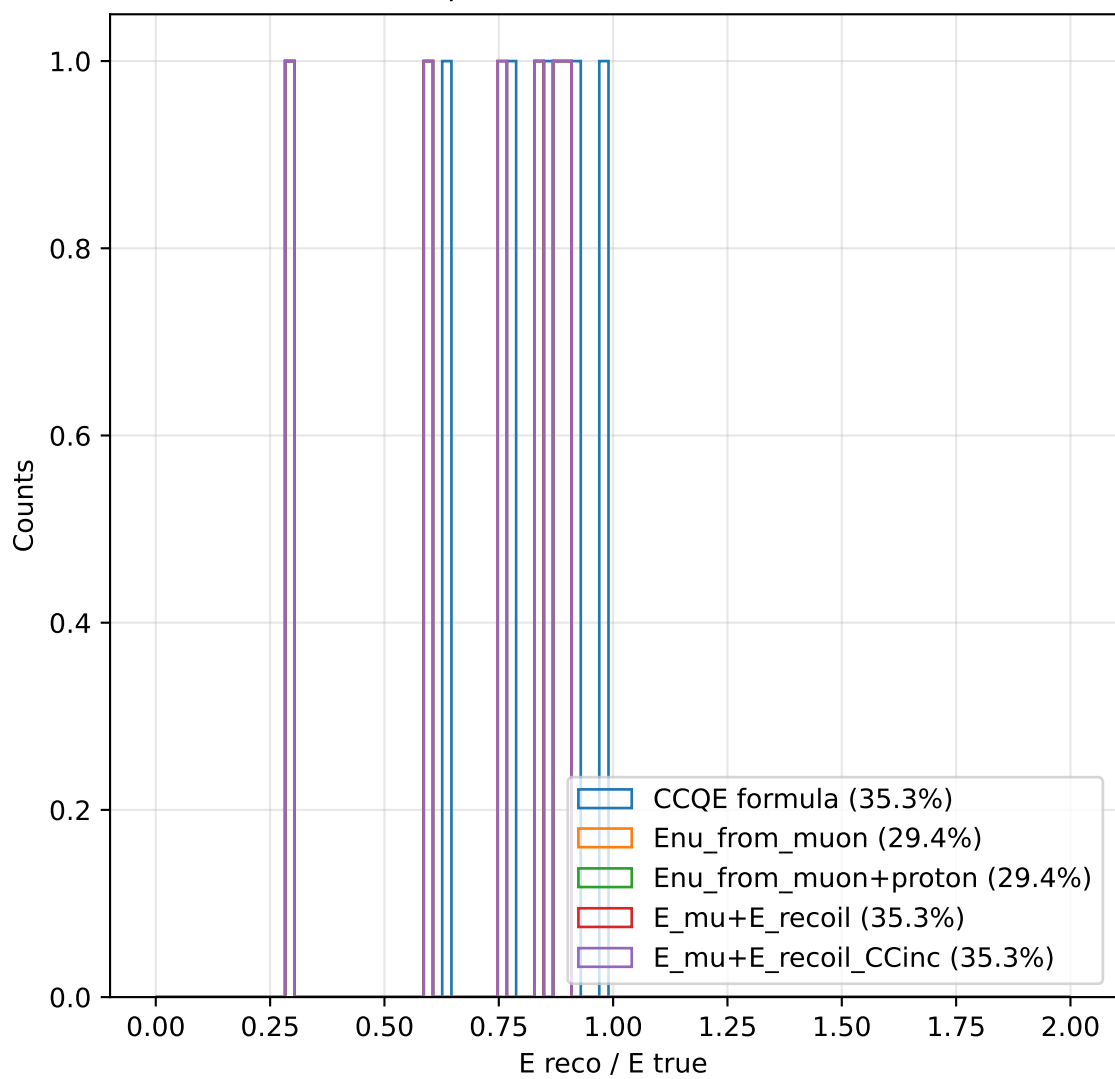
E reco / E true Distribution - Other
