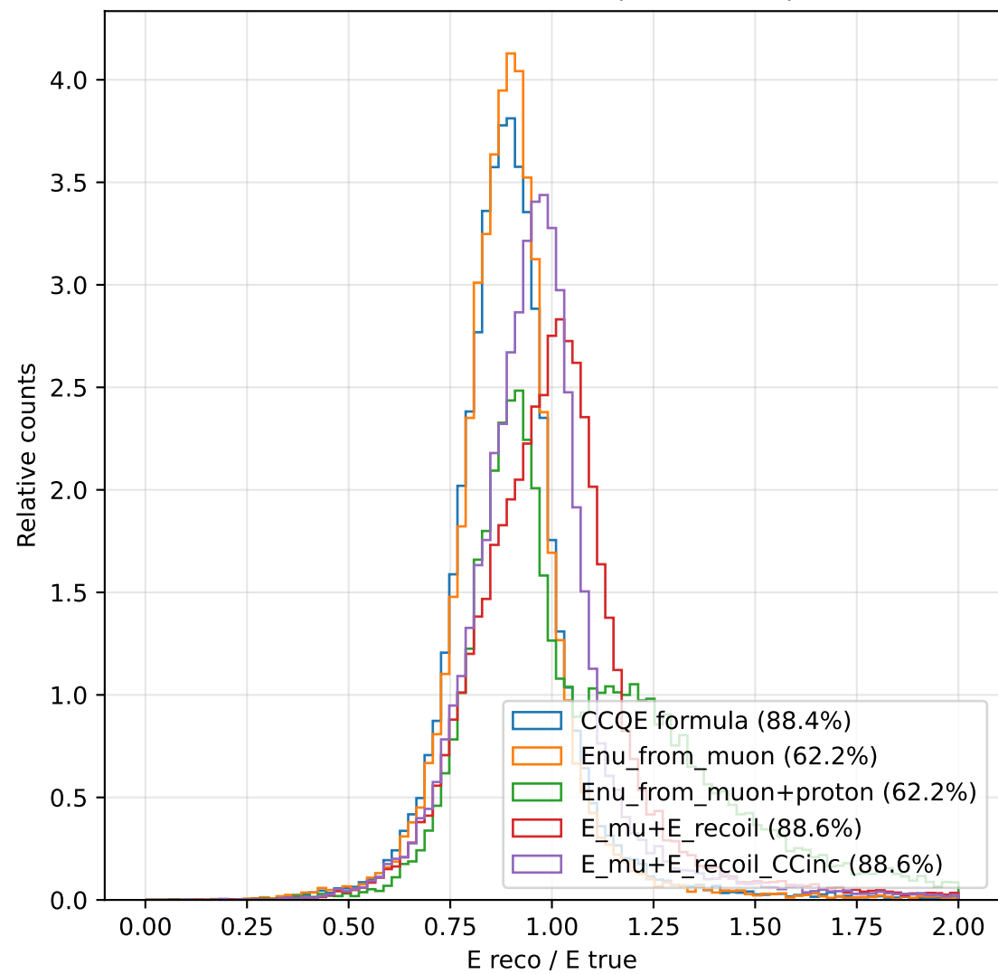
E reco / E true Distribution (normalized) - RES
