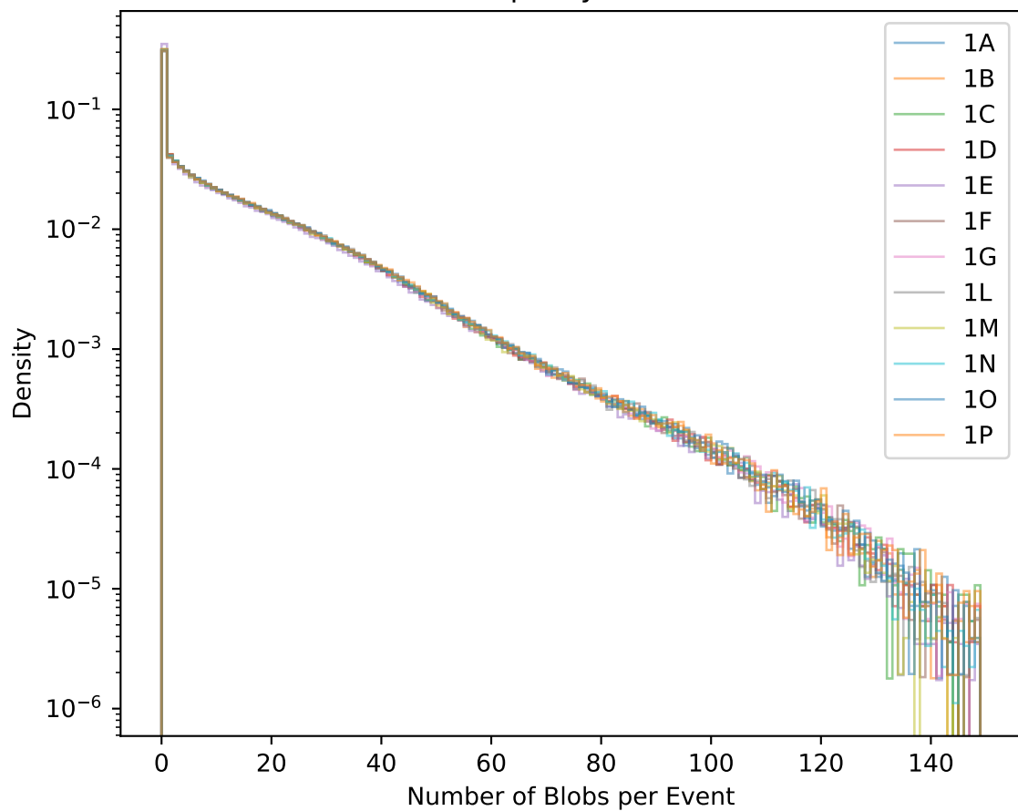
Muon Multiplicity Distribution
