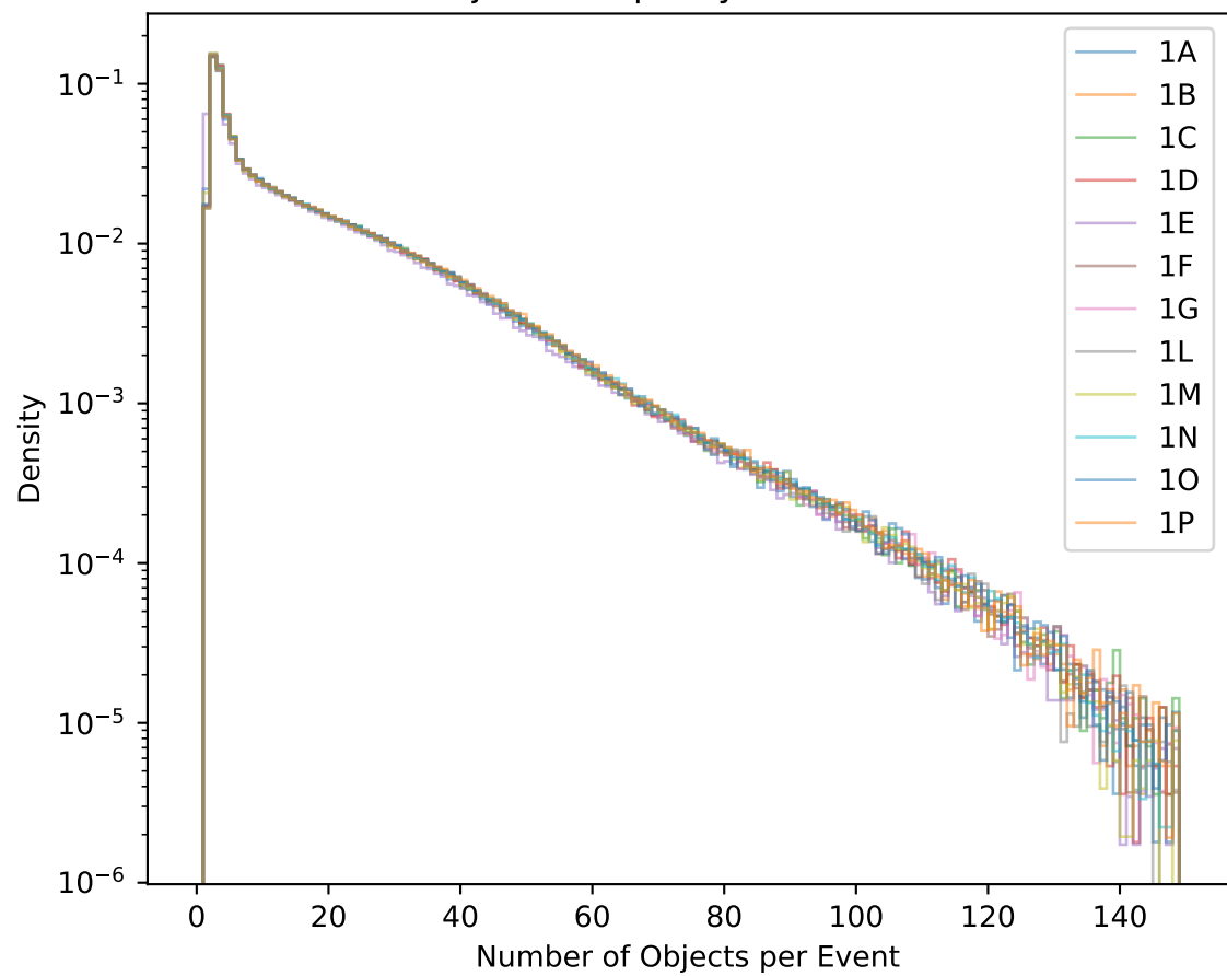
Object Multiplicity Distribution
