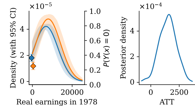
Logistic regression
