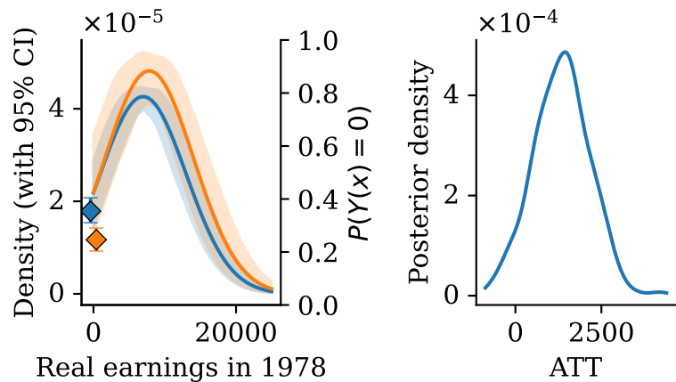
Bayesian bootstrap
