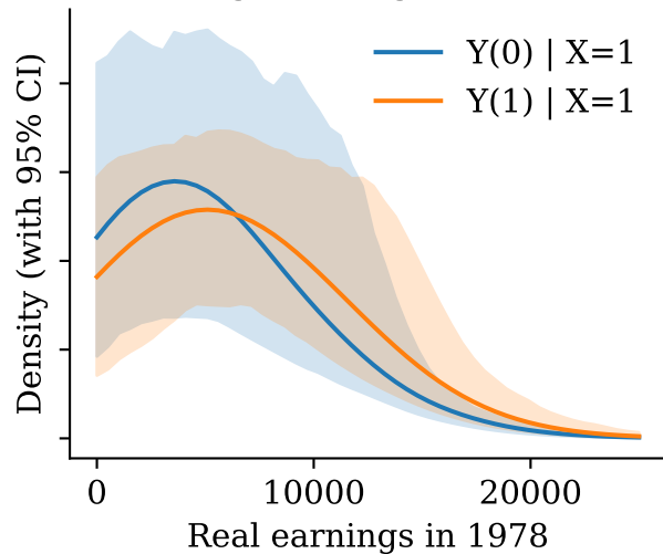
Logistic regression
