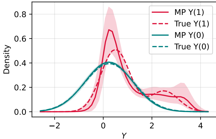
T-Learner
