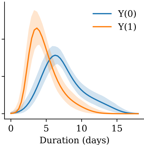
T-learner
