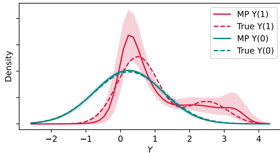
Scenario 1: T-Learner
