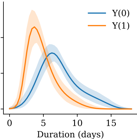
T-learner
