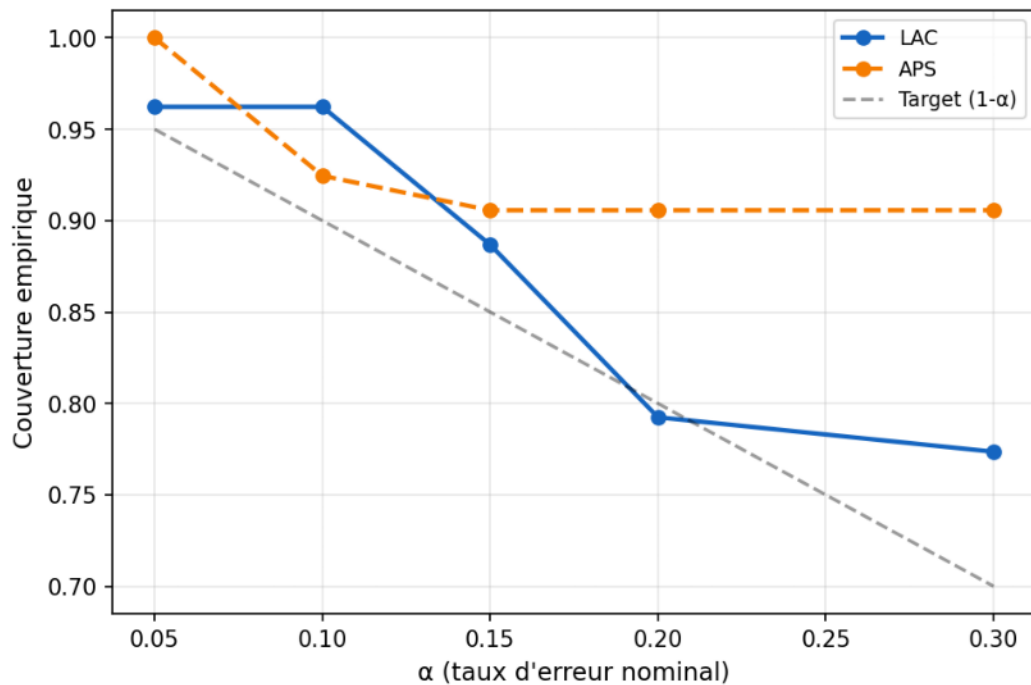
Couverture vs \alpha
