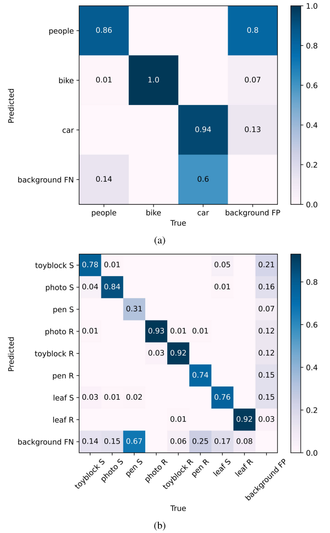
Fig. 7. Illustration of the classification confusion matrix. (a) HOD3K dataset. (b) HOD-1 dataset.
