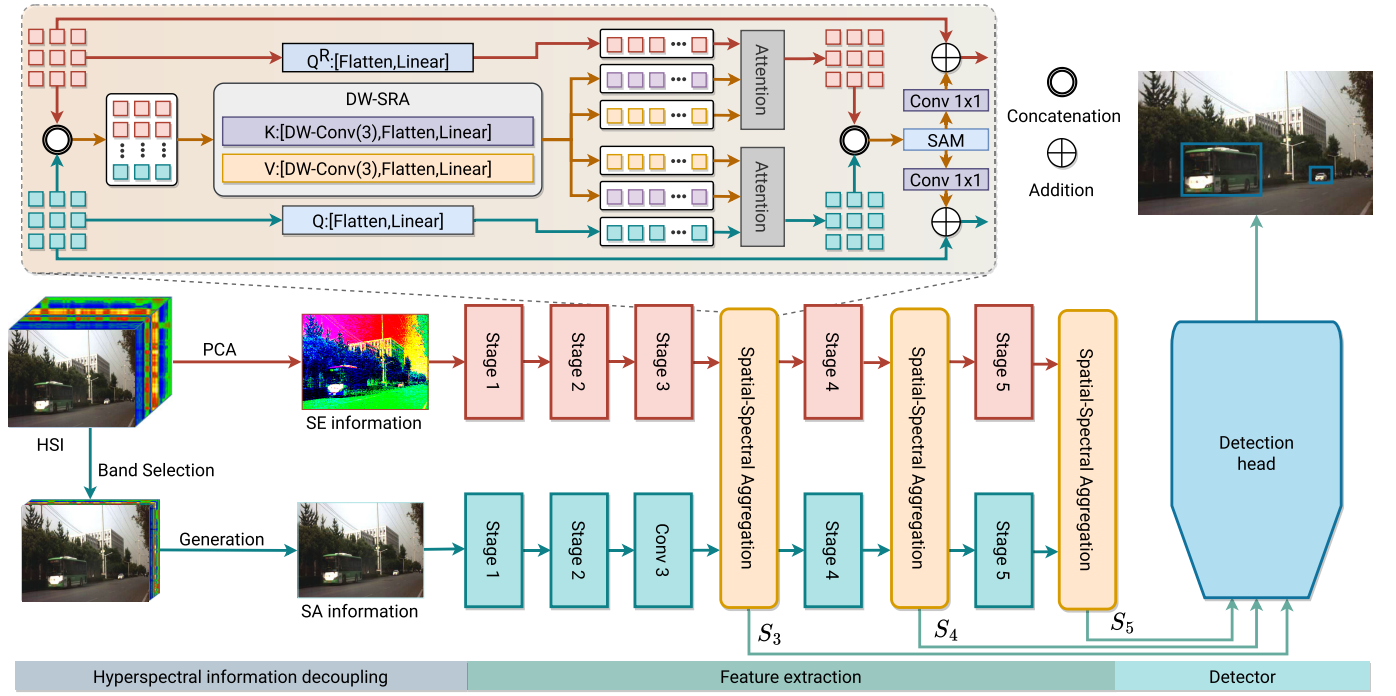
Fig. 3. Structure of S2ADet. It contains a HID module, a two-stream network, a SSA module, and a one-stage detection head. The HID module is used to remove redundant information. We designed a two-stream feature extraction network embedded with SSA modules for interacting with the spectral and spatial dimensional features of HSIs.
