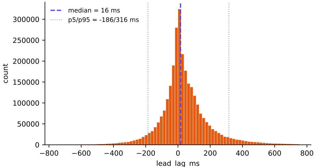
Lead--Lag Distribution (unified, n=2,936,031)
