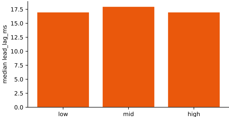
Lead--Lag by Disagreement Regime
