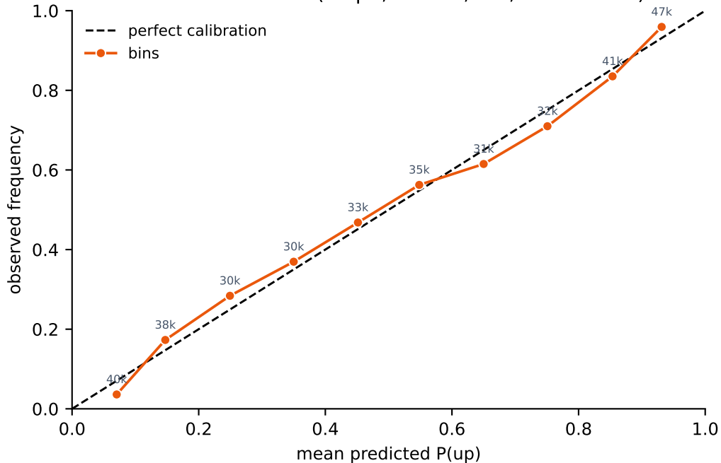
Calibration Curve (step3, n=357,390, ECE=0.027)
