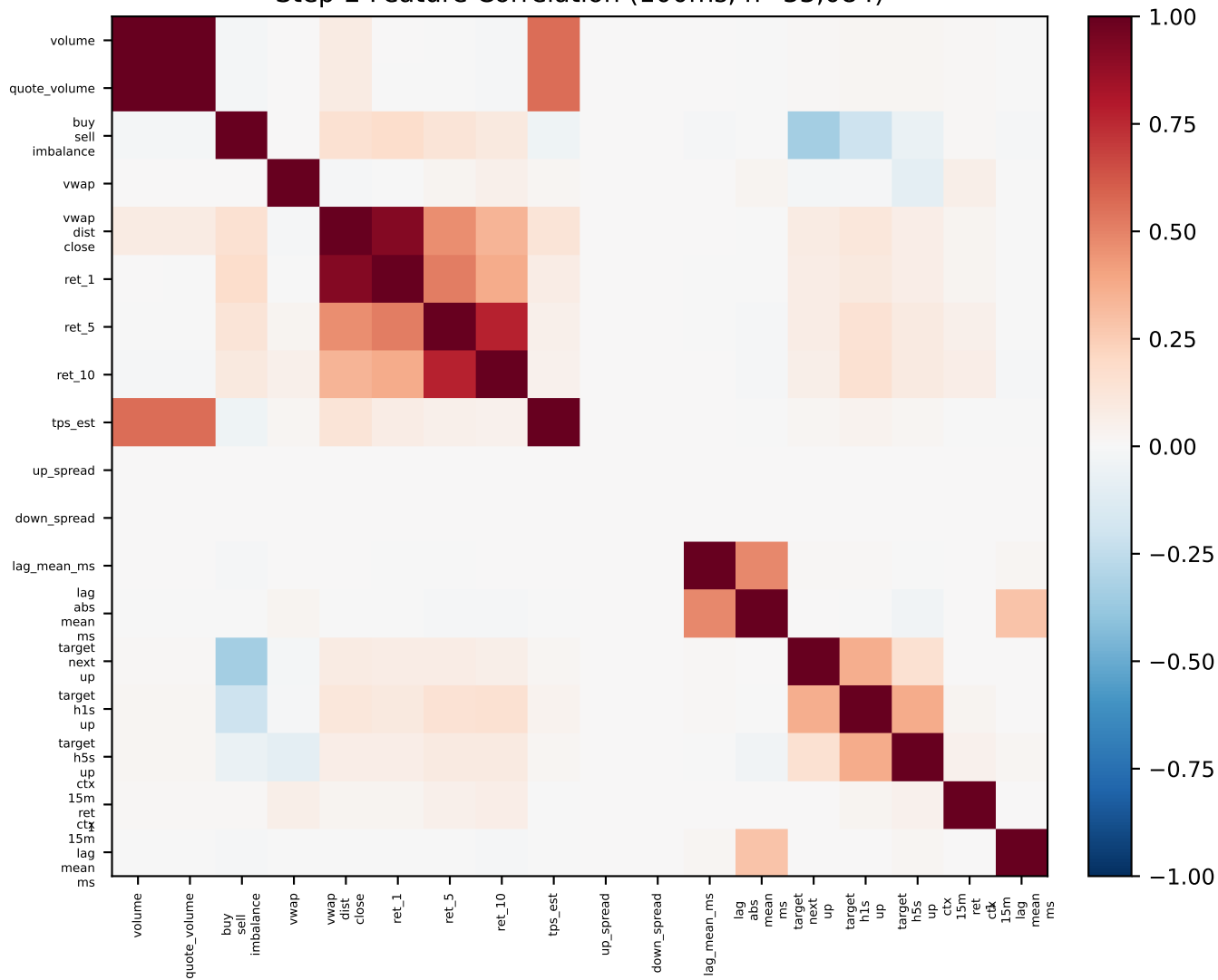
Step-2 Feature Correlation (100ms, n=33,084)
