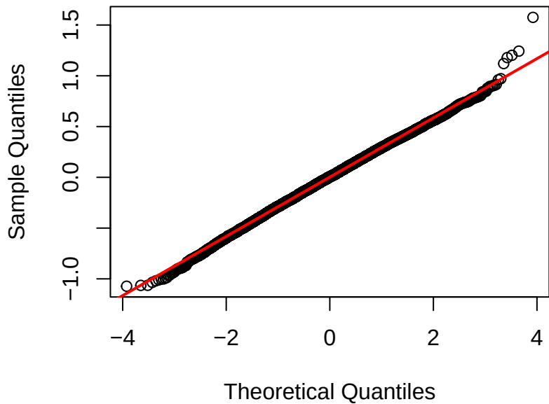
Normal Q-Q Plot of Residuals
