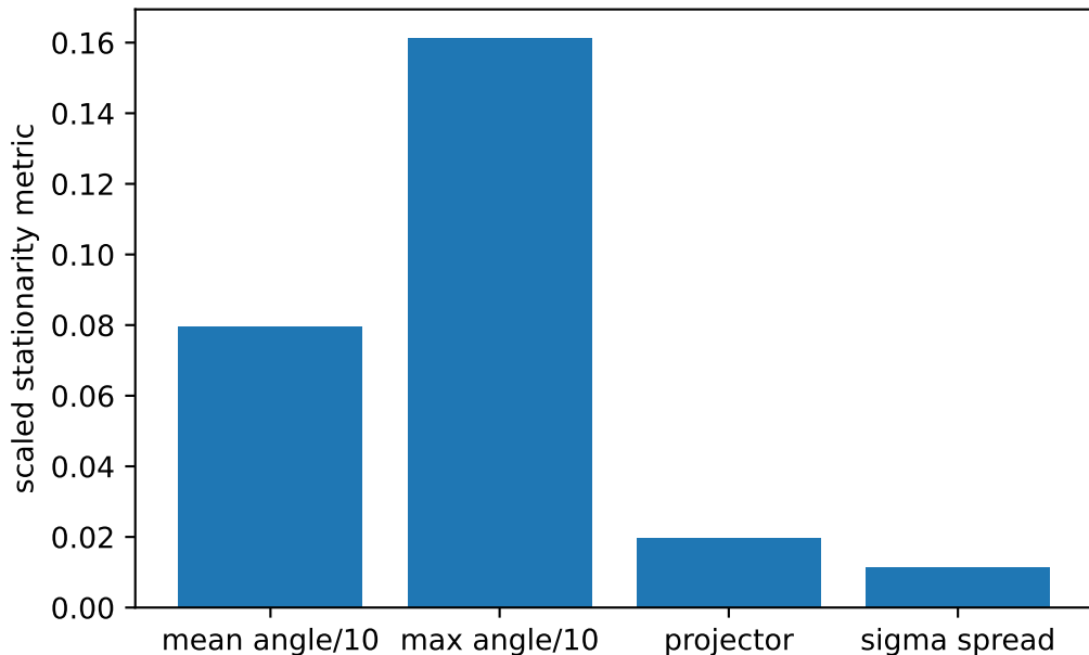
Fig. S5 | Dominant mode is stable across historical fields
