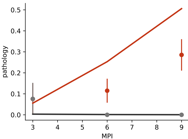
ill: delta-PC1=3.65
