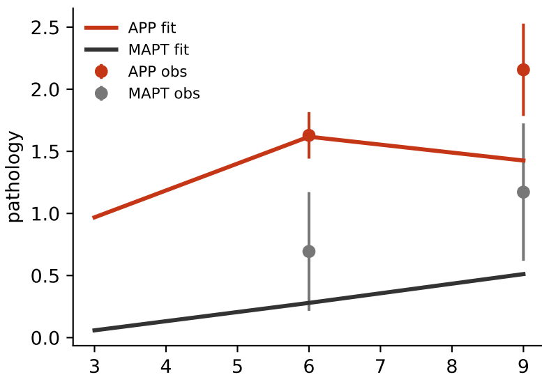
ill: delta-PC1=3.65
