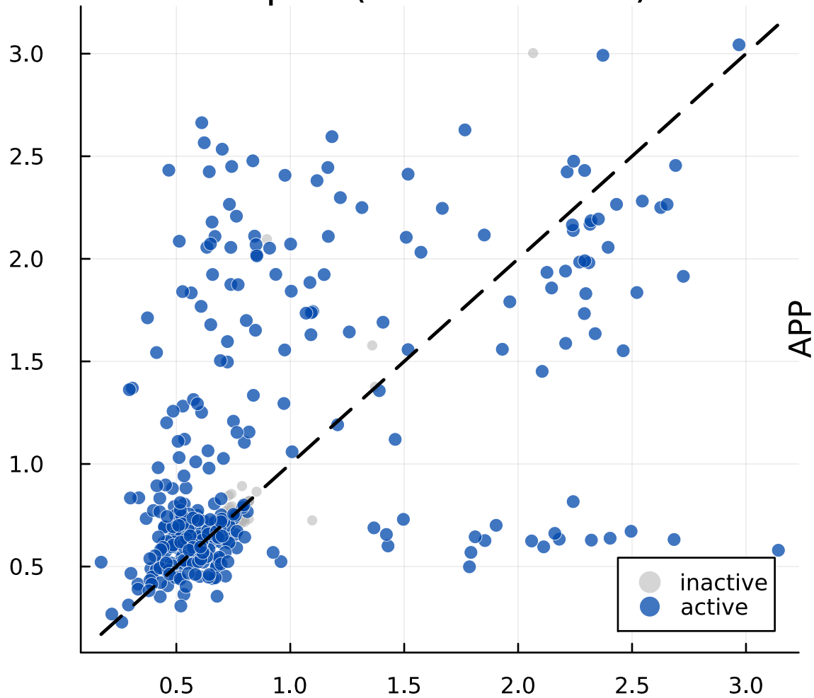
alpha (active r=0.51 )
