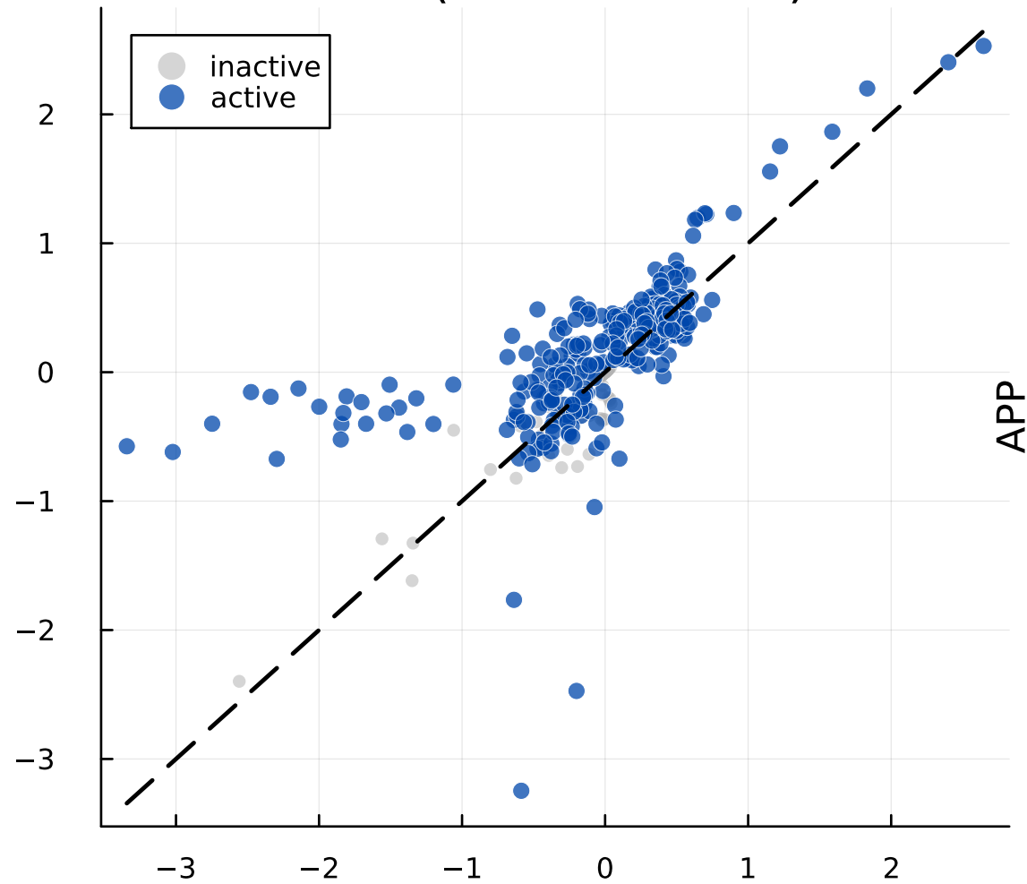
SYN REGION-RF: APP vs MAPT beta (active r=0.66 )
