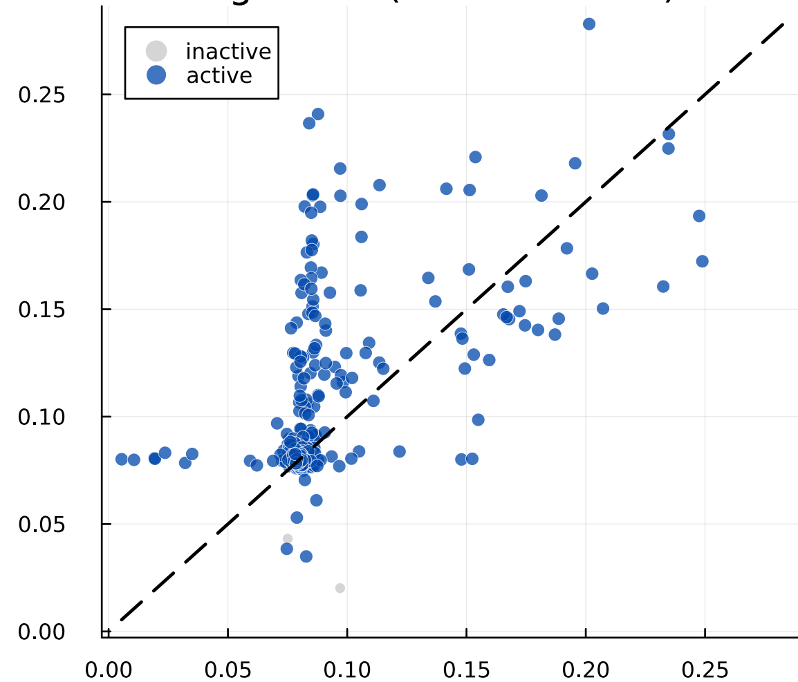
gamma (active r=0.59 )
