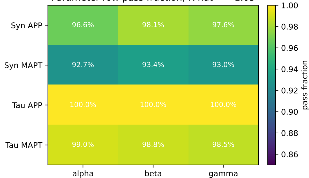
Parameter-row pass fraction, R-hat <= 1.05
