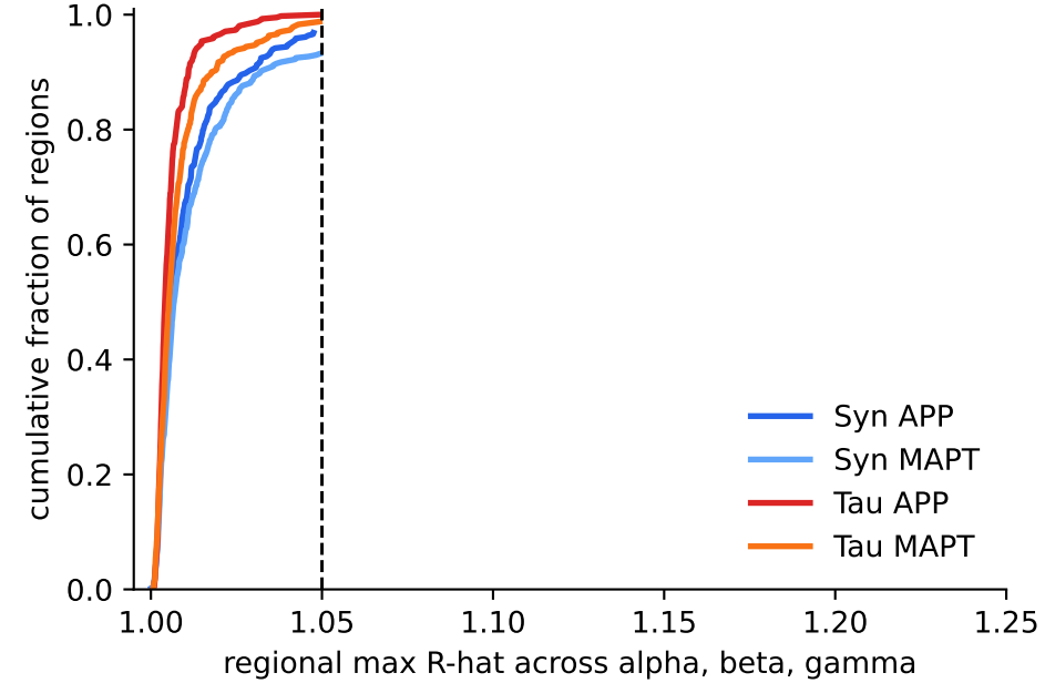
Distribution of regional R-hat
