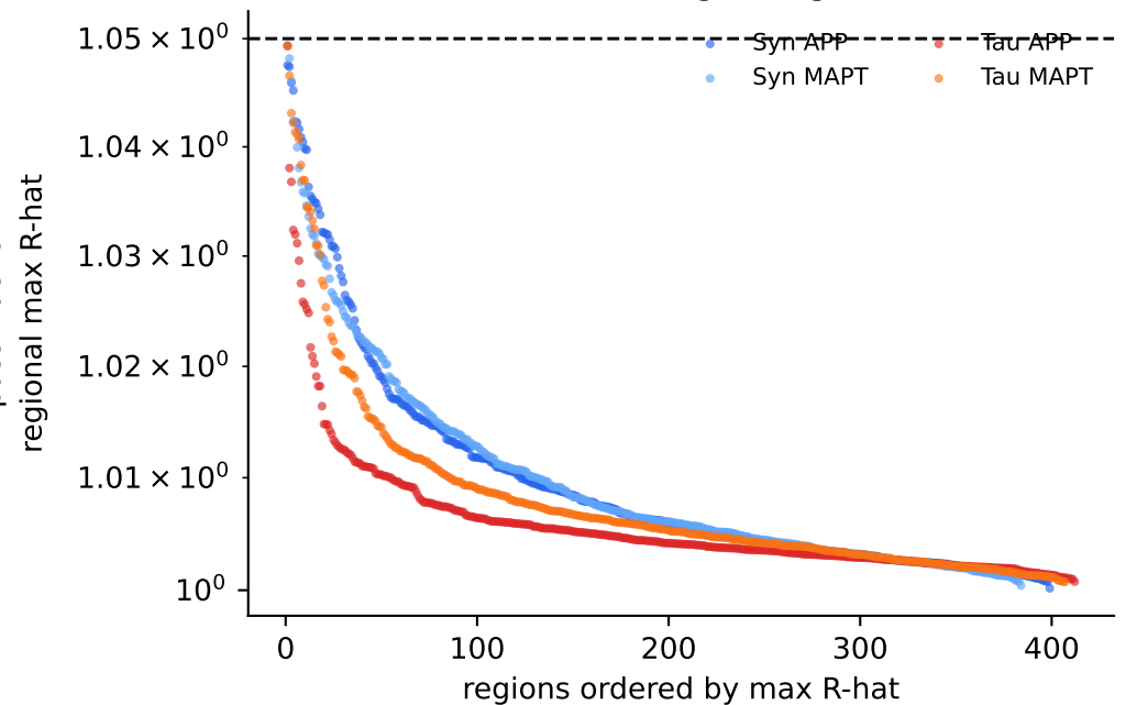
Tail of non-converged regional fits
