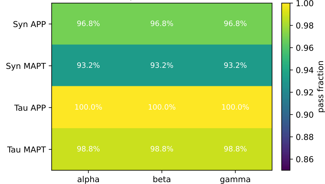
Parameter-row pass fraction, R-hat \leq 1.05
