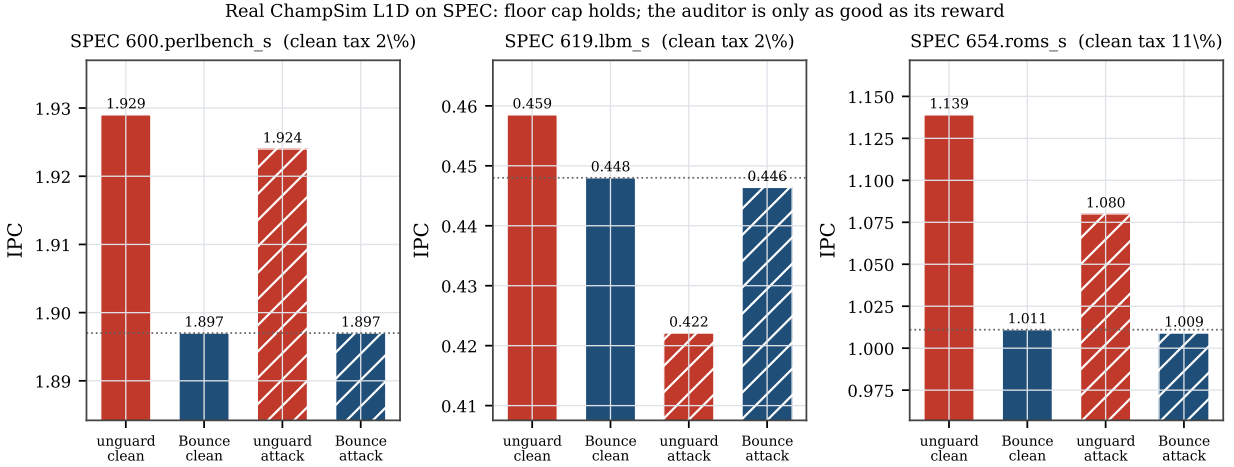
Figure 18: Bouncer as a real ChampSim L1D prefetcher across a SPEC suite. On every trace Bouncer ends at the prefetch-off floor (the cap), bounding the corruption attack’s worst case (lbm: 7.9% unguarded loss cannot reach the gated victim). The per-set cache-hit reward proxy sets the clean tax (1.7–11%): roms shows the failure mode—a genuinely-helpful prefetcher under-credited and over-gated. Swapping to the controller’s own reward does not fix this (only 11.2% \rightarrow 9.7%); a prefetcher’s benefit is not set-local, so set-dueling needs a longer epoch or a set-local signal (replacement is the set-local case—though a real cache’s stateful reward is a further boundary; see Section 11.10).
