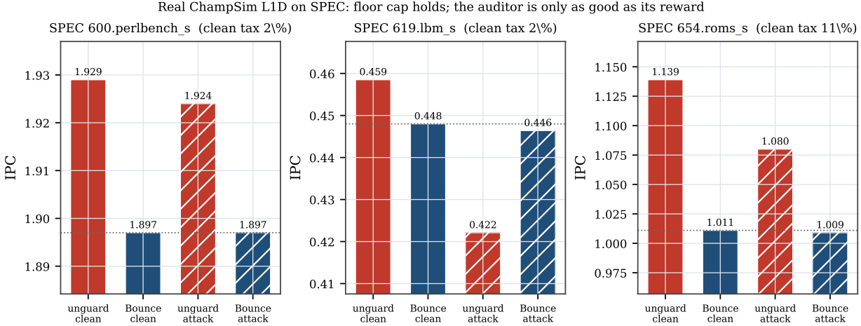
Figure 16: Bouncer as a real ChampSim L1D prefetcher across a SPEC suite. On every trace Bouncer ends at the prefetch-off floor (the cap), bounding the corruption attack’s worst case (lbm: 7.9% unguarded loss cannot reach the gated victim). The per-set cache-hit reward proxy sets the clean tax (1.7–11%): roms shows the failure mode—a genuinely-helpful prefetcher under-credited and over-gated. Swapping to the controller’s own reward does not fix this (only 11.2% \rightarrow 9.7%); a prefetcher’s benefit is not set-local, so set-dueling needs a longer epoch or a set-local signal (replacement is the set-local case—though a real cache’s stateful reward is a further boundary; see Section 11.10).
