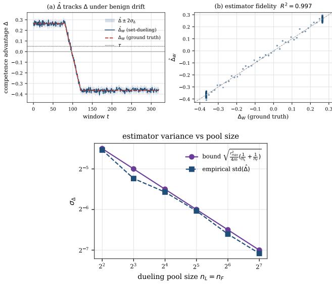
Fig. 3: P0. (top) \hat{\Delta} tracks ground-truth \Delta ( R^2=0.997 ); (bottom) empirical \text{std}(\hat{\Delta}) matches the bound eq. (2).
