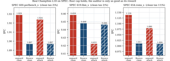
Fig. 13: Bouncer as a real ChampSim L1D prefetcher across a SPEC suite. On every trace Bouncer ends at the prefetch-off floor (the cap), bounding the corruption attack’s worst case (lbm: 7.9% unguarded loss cannot reach the gated victim). The per-set cache-hit reward proxy sets the clean tax (1.7–11%): roms shows the failure mode—a genuinely-helpful prefetcher under-credited and over-gated. The fix is the controller’s own in-silicon reward.
