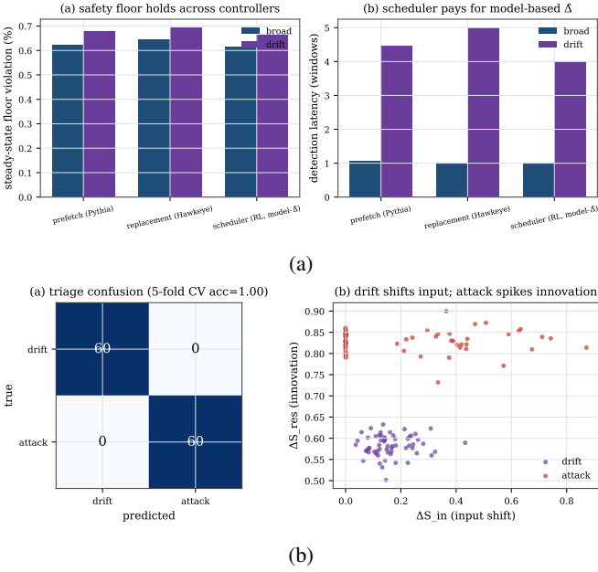
Fig. 7: P3. (a) the floor holds across controller classes; (b) attack-vs-drift triage (acc 1.0).
