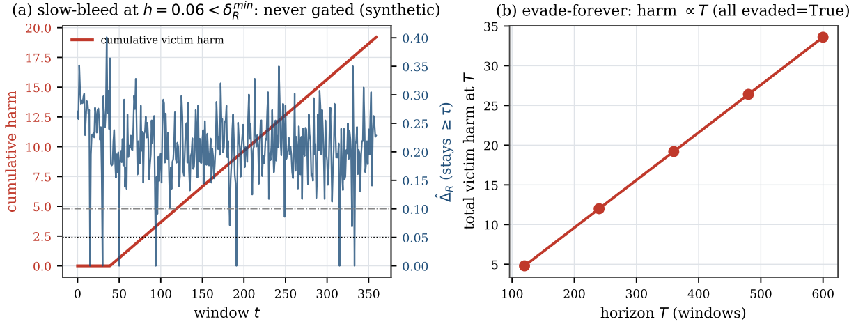
Figure 3: The coverage hole, demonstrated (controlled harness, real Bouncer region dueling). (a) a slow-bleed at h < \delta_R^{\min} accumulates unbounded victim harm while \hat{\Delta}_R \geq \tau and no alarm fires; (b) it evades at every horizon, so total harm \propto T . The closed-form floor is \delta_R^{\min}(B) = k\sigma_R \propto 1/\sqrt{B} (0.19, 0.13, 0.094, 0.066 for per-pool leader counts n_{L,R}=2, 4, 8, 16 ): more leader budget shrinks the hole but never closes it.
