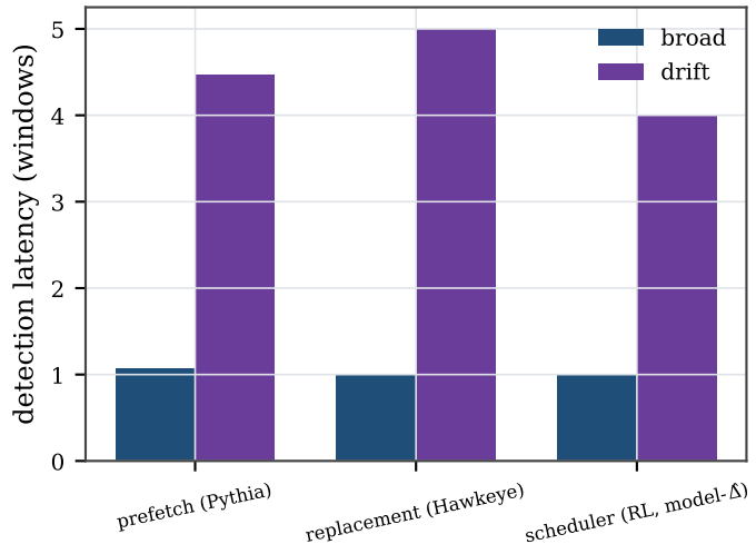
(b) scheduler pays for model-based \Delta
