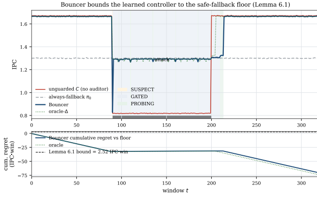
Fig. 5: P1. Bouncer bounds the controller to the fallback floor under attack and re-trusts after it ends; the ungarded controller crashes below the floor.
