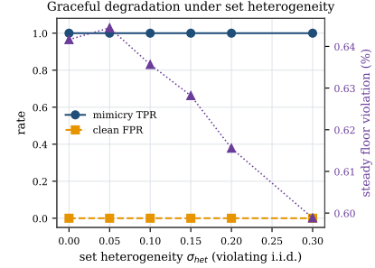
Fig. 11: Graceful degradation when the i.i.d.-set assumption is violated: under set heterogeneity \sigma_{het} up to 0.30, mimicry TPR stays 1.0 and the floor holds; only detection latency drifts up ( 1.0 \rightarrow 1.7 windows).
