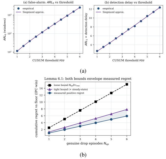
Fig. 13: Theory. (a) ARL matches Siegmund; (b) the safety-floor bound envelopes measured regret.
