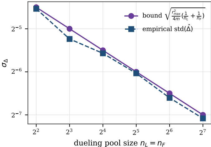
estimator variance vs pool size
