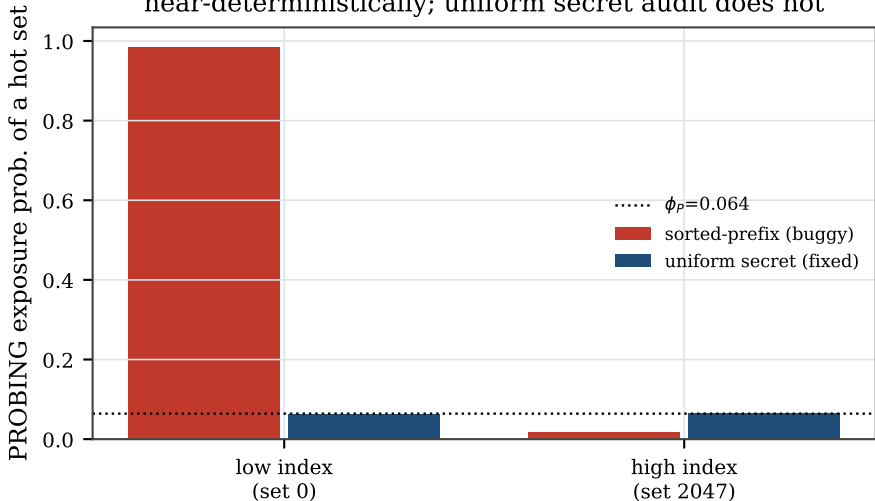
Sorted-prefix audit exposes low-index sets near-deterministically; uniform secret audit does not
