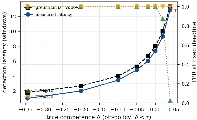
Latency tracks H/(K-\Delta) ; fixed-deadline TPR falls near \tau
